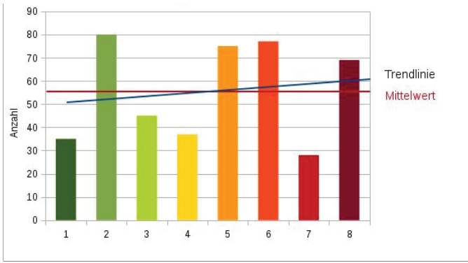
Figure 4. Bar graph in 8 meteorosensitivity steps (abscissa) due to its quantity (quantity, see ordinate “Anzahl”; mean & trend lines inserted, see “Trendlinie” and “Mittelwert”).
